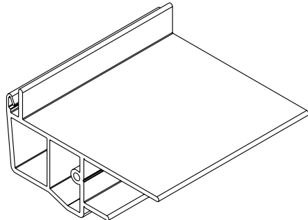
Brickmould Extrusion #1084
