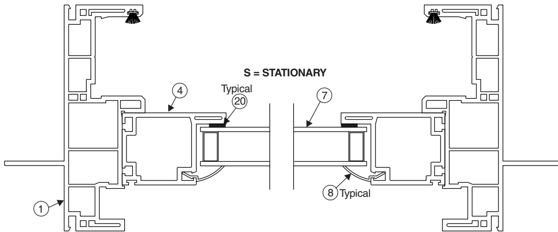
Stationary and Transom Top View
