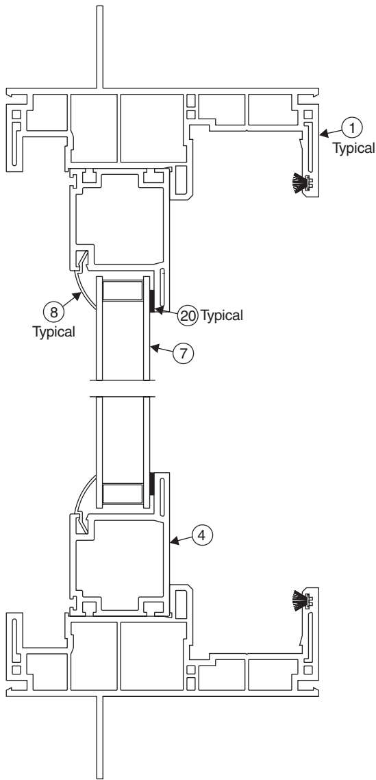
Stationary and Transom Side View
