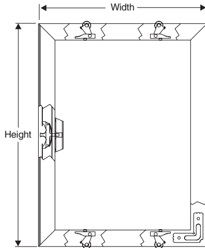
#11) Patio Door Screen (Exterior View) - #914 (Screen shown is for an XO Door)
