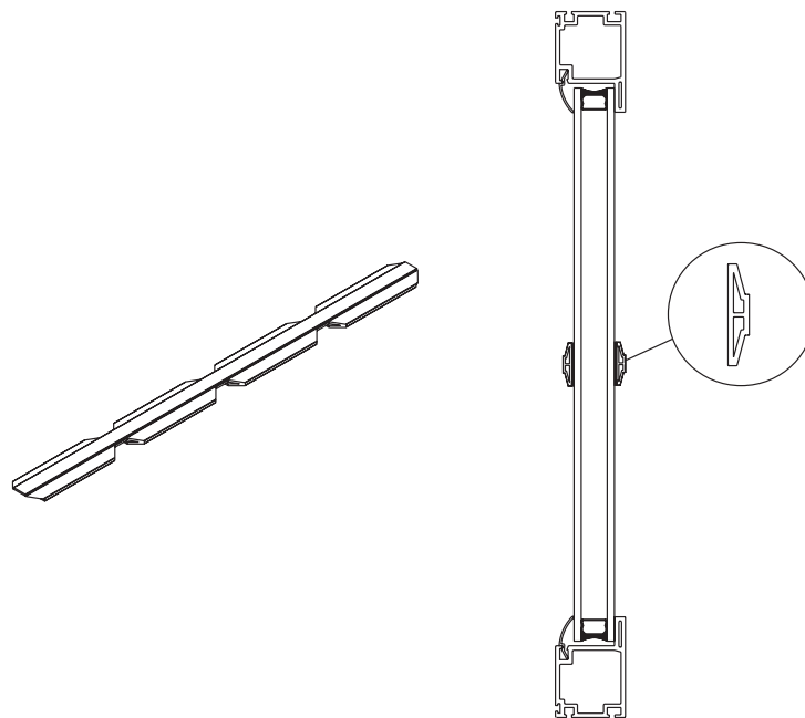
Simulated Divided Light (SDL)
