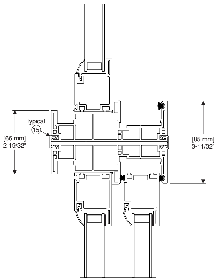
Horizontal Stack Detail
