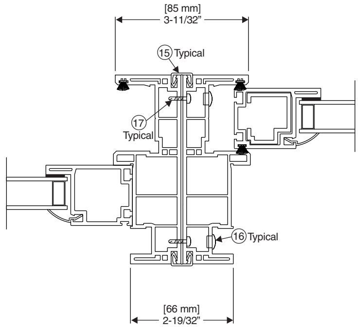
Vertical Mull Detail
