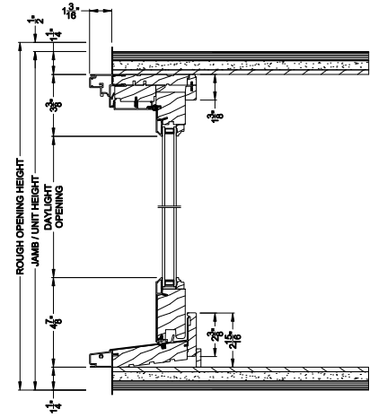
PREMIUM DOUBLE HUNG 45° A-BAY (8120) Vertical Section - Picture Center
