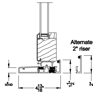
CONTEMPORARY 2-1/4" MULTI-SLIDE PATIO DOOR (8722) Vertical Section - with Sill Riser - 1 or Bi-parting 2 Panel Door
