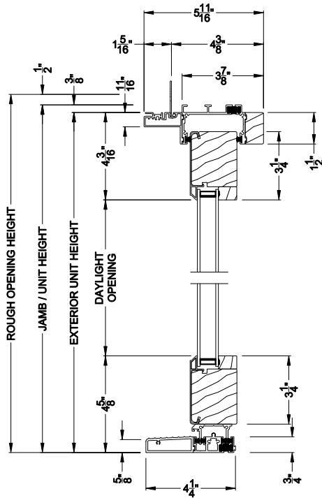
CONTEMPORARY 2-1/4" MULTI-SLIDE PATIO DOOR (8722) Vertical Section - Standard Sill - 1 or Bi-parting 2 Panel Door
