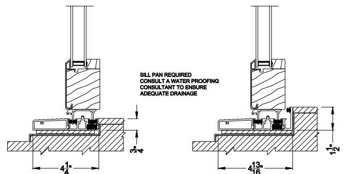
CONTEMPORARY 2-1/4" MULTI-SLIDE PATIO DOOR (8722) Vertical Section - With sill pan
