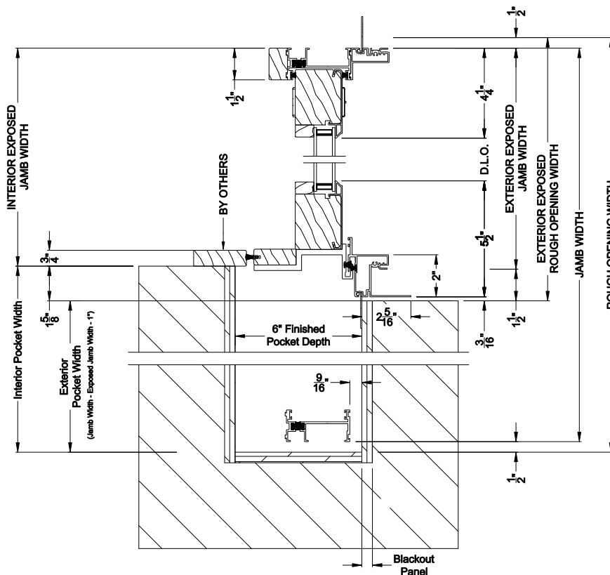
CONTEMPORARY 2-1/4" MULTI-SLIDE PATIO DOOR (8722) Horizontal Section - Bi-parting stiles
