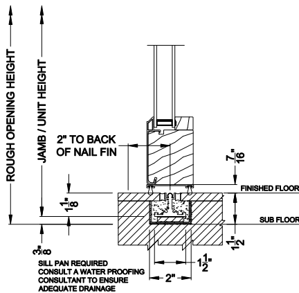
CONTEMPORARY 2-1/4" MULTI-SLIDE PATIO DOOR (8722) Vertical Section - with T-track sill - 1 or Bi-parting 2 Panel Door
